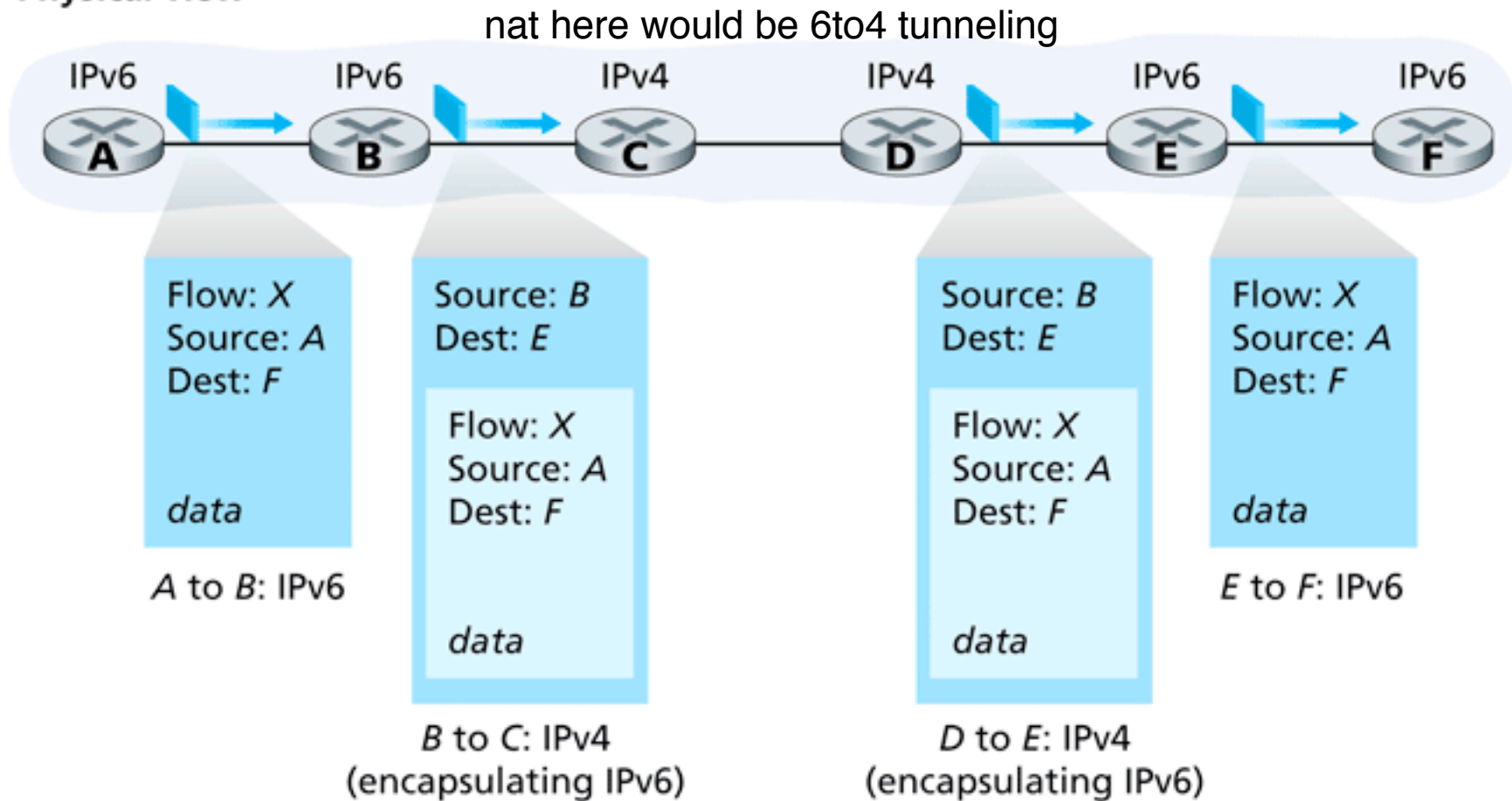
Figure 4.26 ♦ Tunneling
