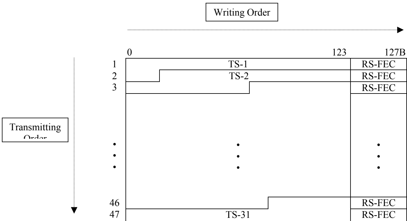
Figure 10: Interleaved Transport Stream (Reed-Solomon FEC)
