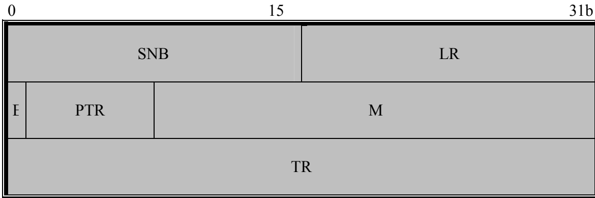
Figure 16: RTP FEC Header Extension
