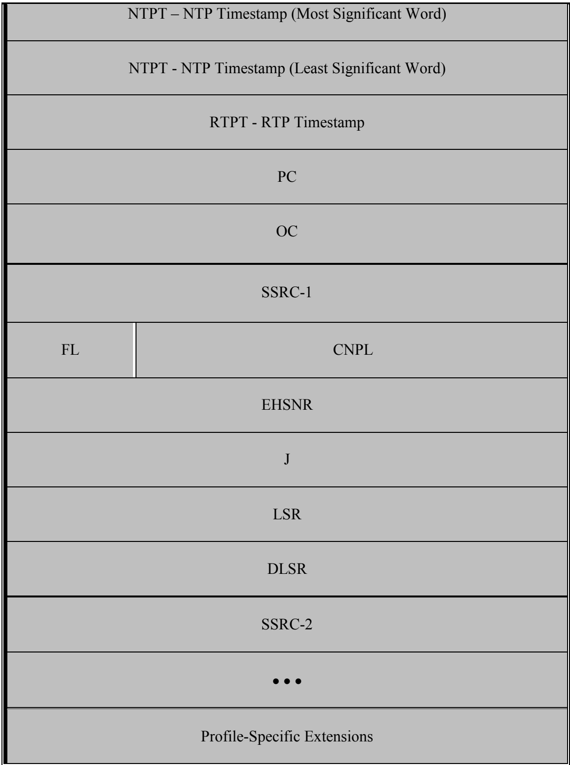
Figure 20: RTCP Sender Report (SR) Packet
