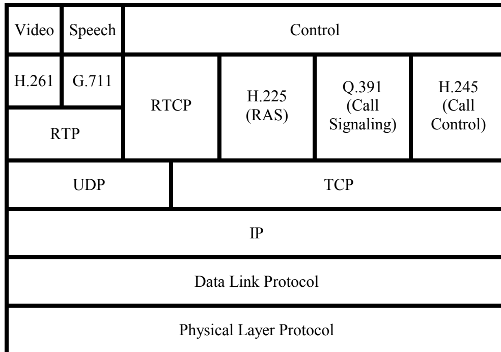
Figure 24: H.323 Protocol Stack.
