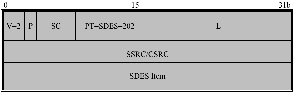
Figure 22: RTCP Source Description (SDES) Packet
