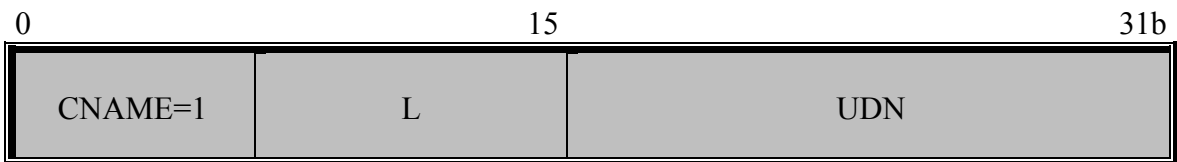
Figure 23: RTCP SDES Canonical End-Point Identifier (CNAME) Item
