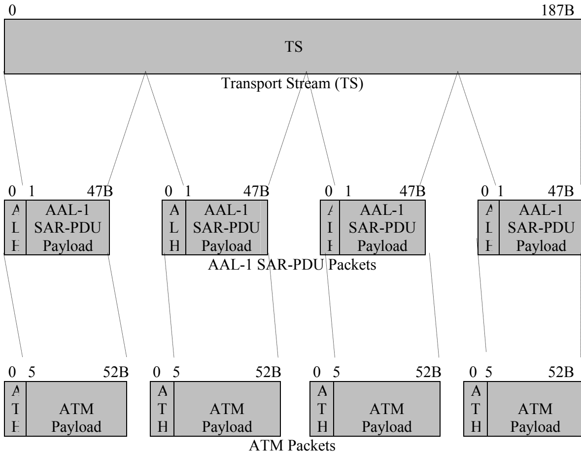
Figure 11: MPEG-2 TS AAL-1 PDU Mapping
