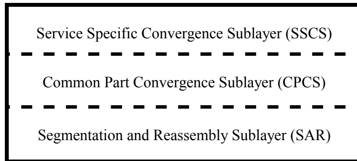
Figure 8: ATM Adaptation Layer (AAL)
