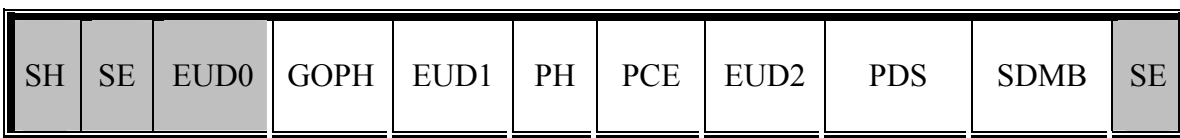
Figure 3: Video Elementary Stream Format
