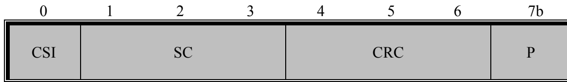
Figure 9: AAL1 SAR-PDU Header
