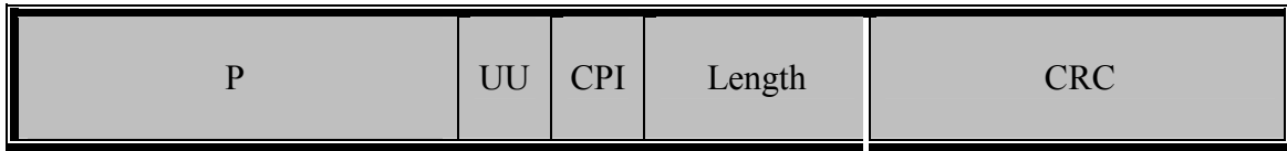
Figure 12: AAL5 CPCS-PDU Trailer
