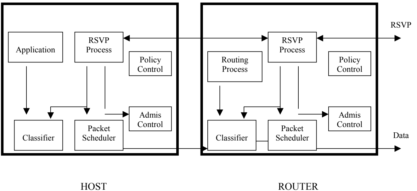
Figure 25: RSVP in Hosts and Routers
