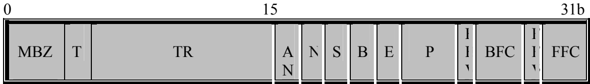
Figure 18: RTP MPEG ES Video-Specific Header
