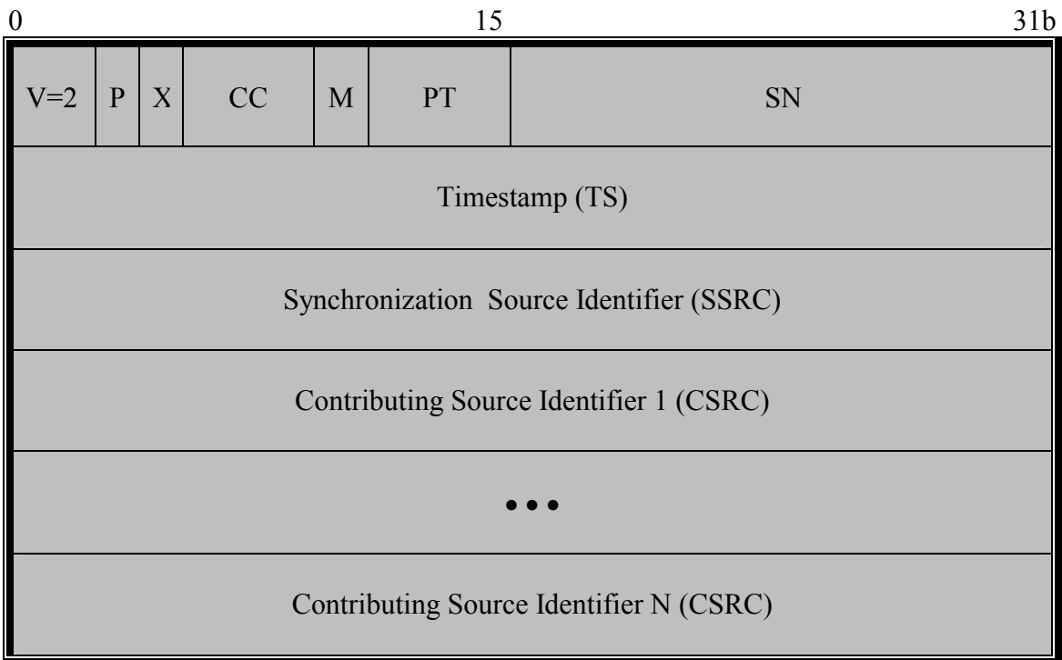
Figure 15: RTP Packet Header
