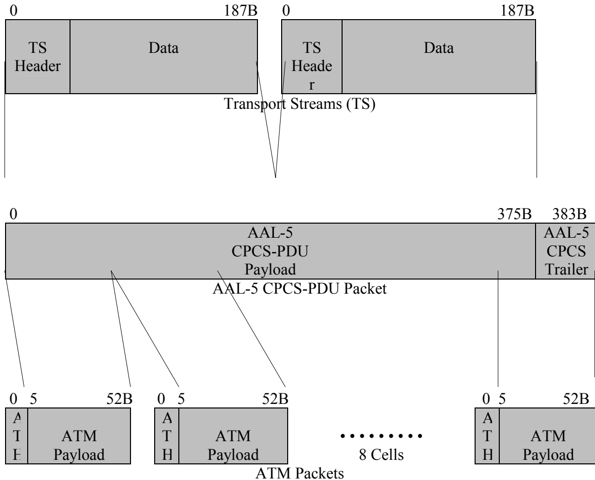
Figure 13: MPEG-2 TS AAL-5 PDU Mapping
